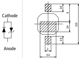
Polarity Recommended Soldering Pattern
