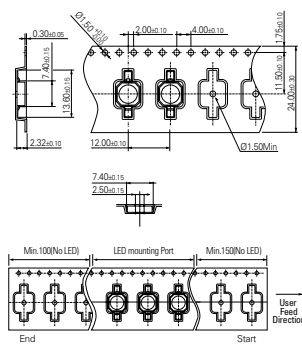
Carrier Tape
