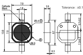
Package Outline
